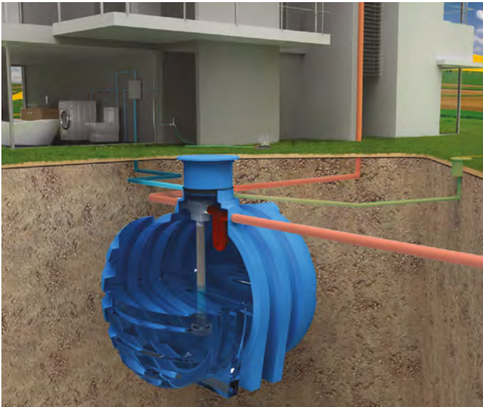
NEPTUN installed with inflow set
